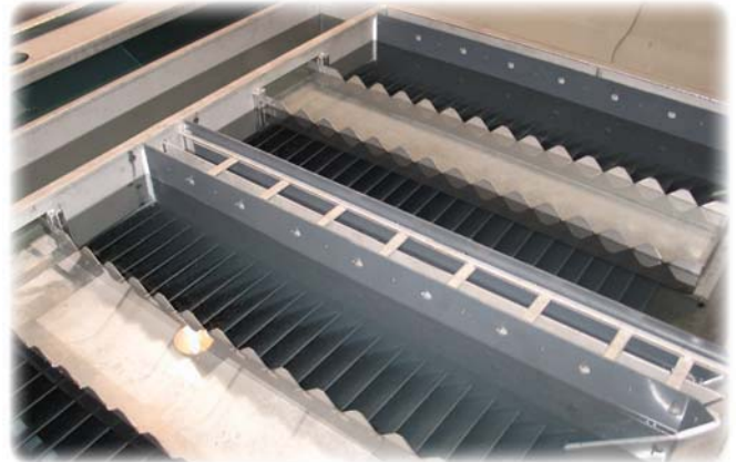
Top view of the lamella plates
